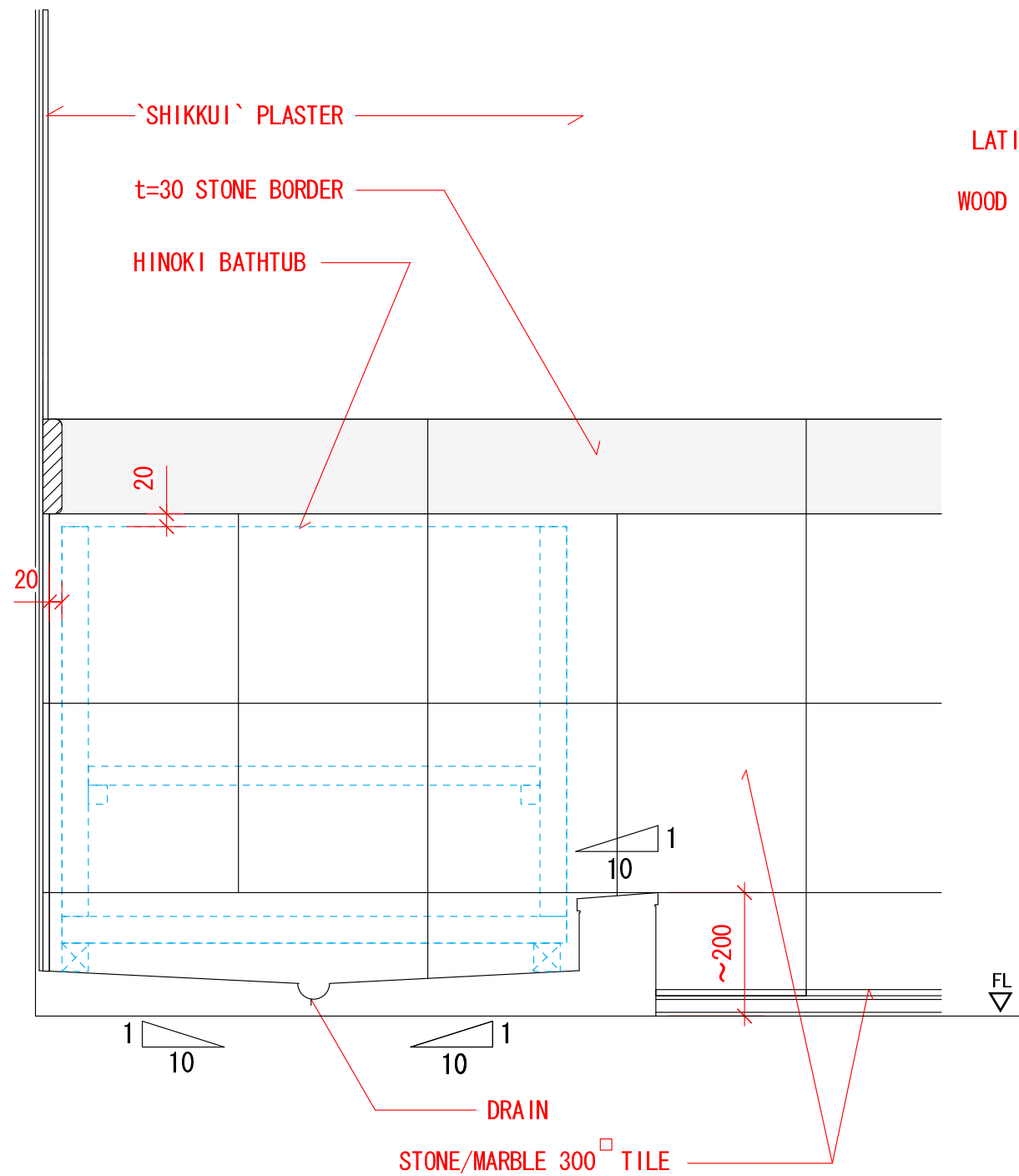
#1 BATHTUB ON CURB DTL.
