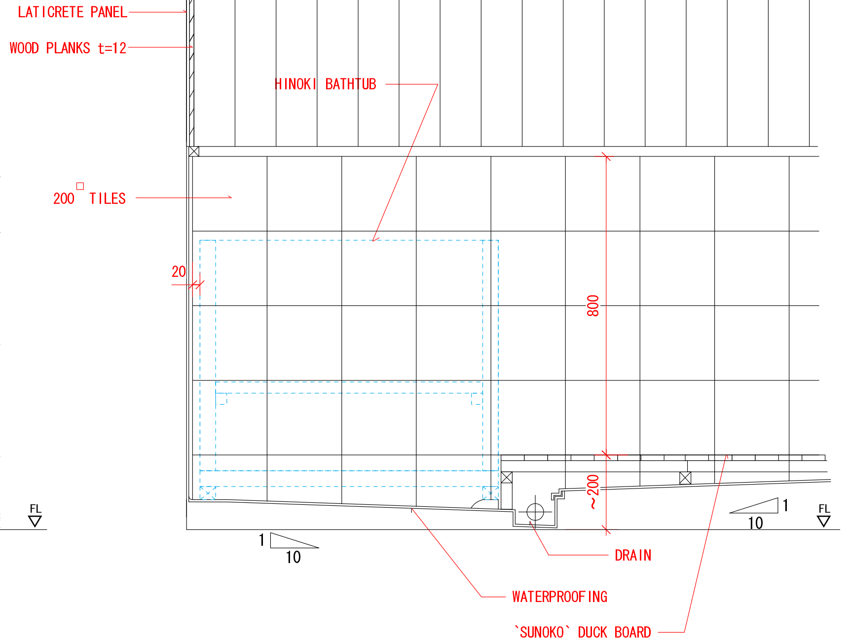
#2 BATHROOM FULL WATERPROOFING DTL.
